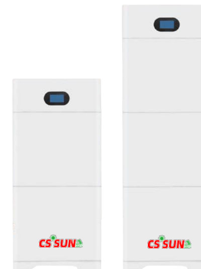
Slim High Voltage Brick Type LiFePO4 Battery Pack 204V 307V 409V 50Ah 10KWh 15KWh,20KWh
