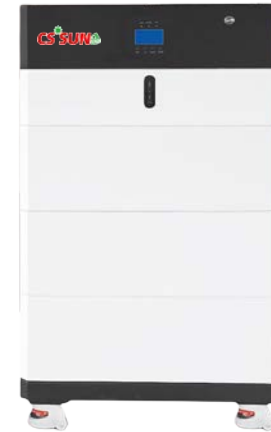
High Voltage Brick All-In-One LiFePO4 Battery + 10KW Inverter 204V50Ah 307V 50Ah,409V50Ah 10KWh 15KWh,20KWh + 10KW
